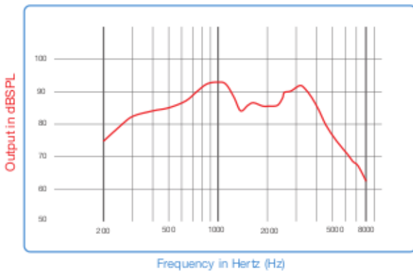
OSPL90 CURVE
